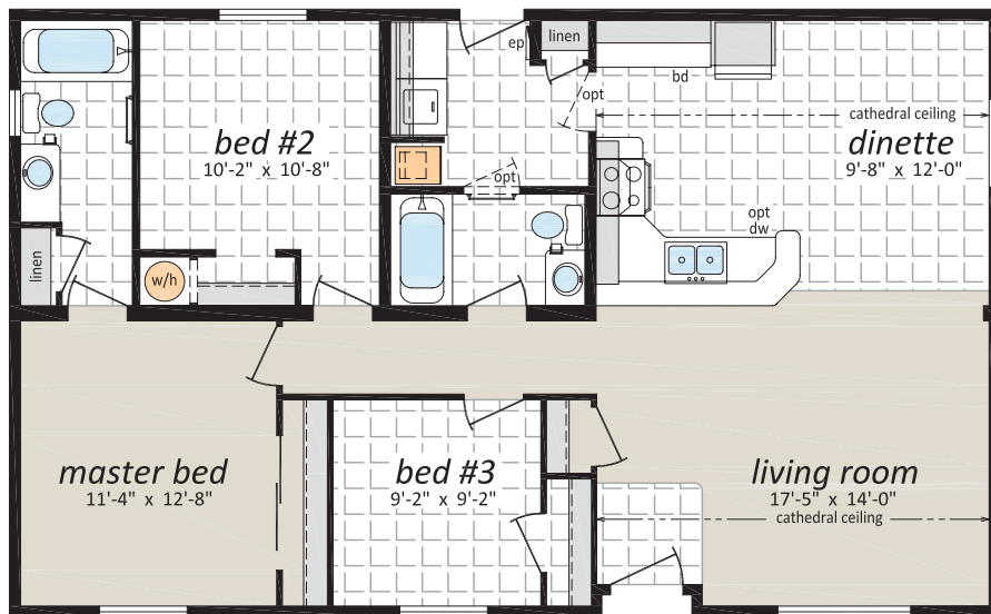
The Galiano, GL-8441 27' x 44' | 1,188 sq. ft.
