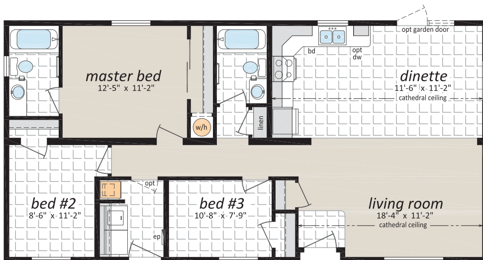
The Utah, GL-4480 24' x 48' | 1,152 sq. ft.
