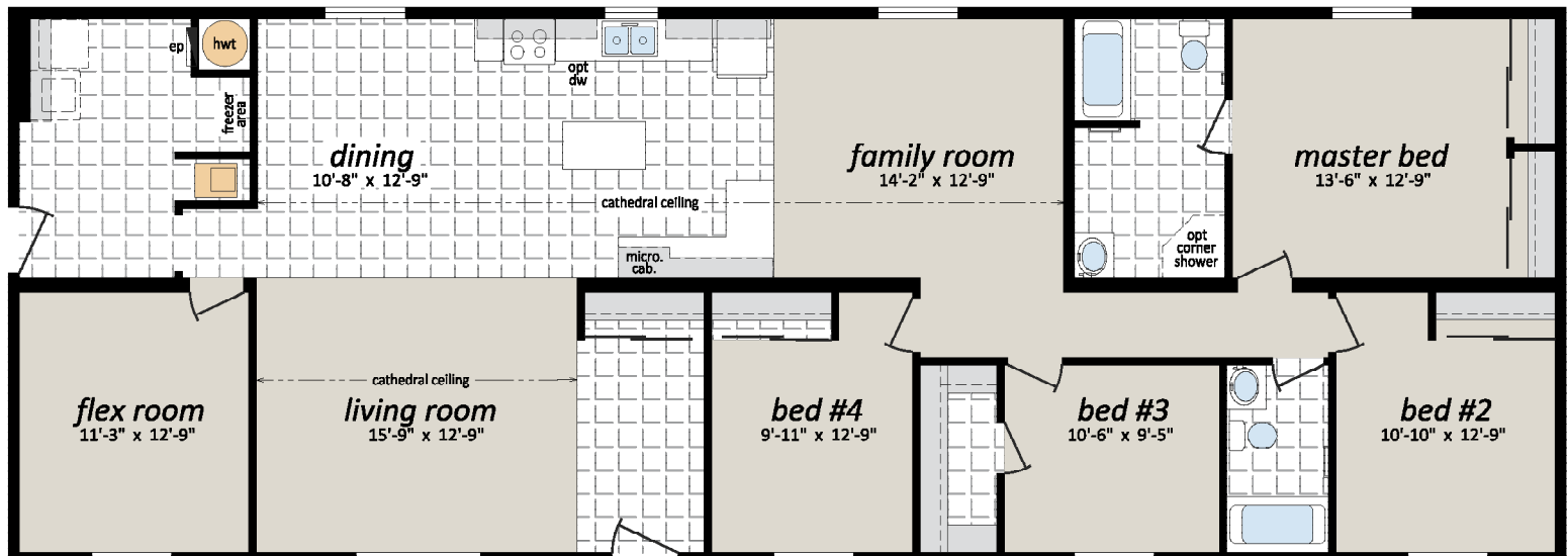
MS-2865 28' x 76', 2,090 sq. ft.
